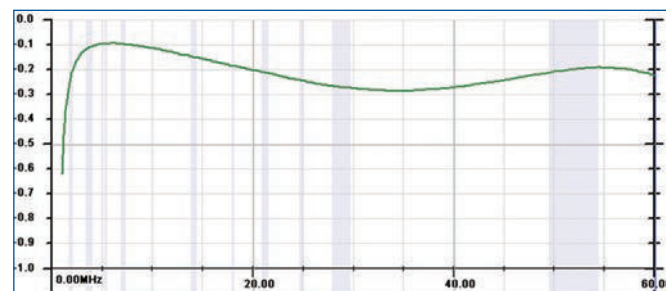
FIGURE 12: Unun through loss in dB.
