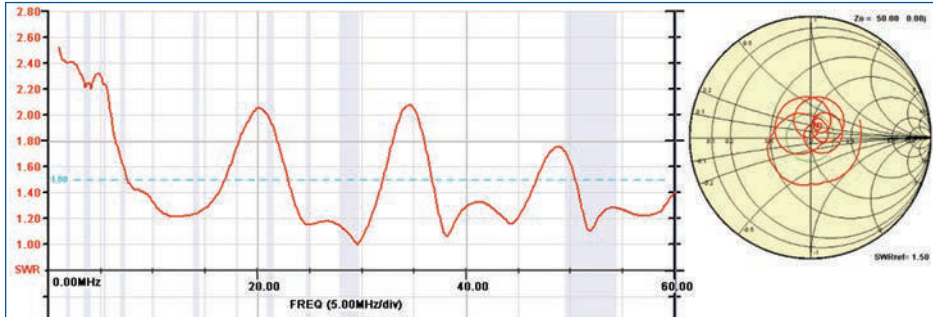
FIGURE 15: Input impedance from 1 to 60MHz, measured at the feedpoint.
